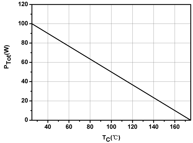
Fig.7-Power Derating
