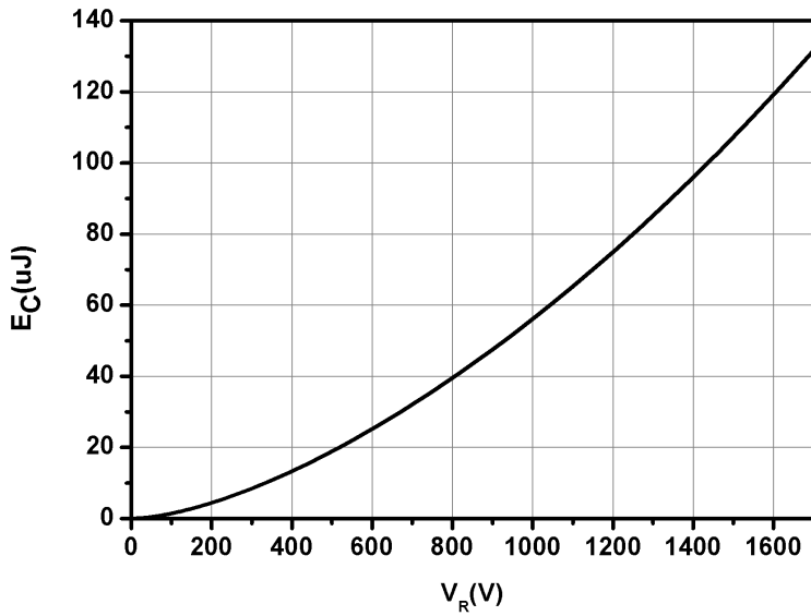
Fig.5-Capacitance Stored Energy
