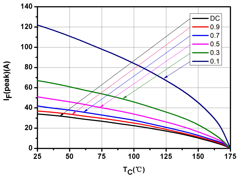
Fig.8-Current Derating
